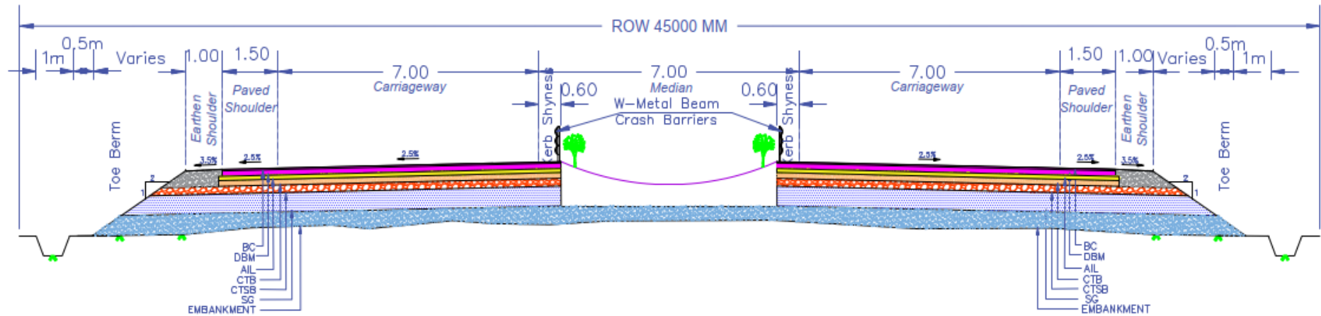
Typical Cross Section for 4-Lane Divided Highway without Service Roads with Depressed Median (New Construction) TCS-01
