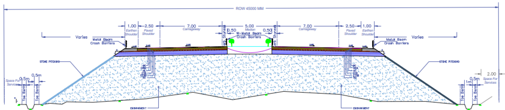
Typical Cross Section for Construction of 4 laning approach to VUP 5m median with earthen embankment.
