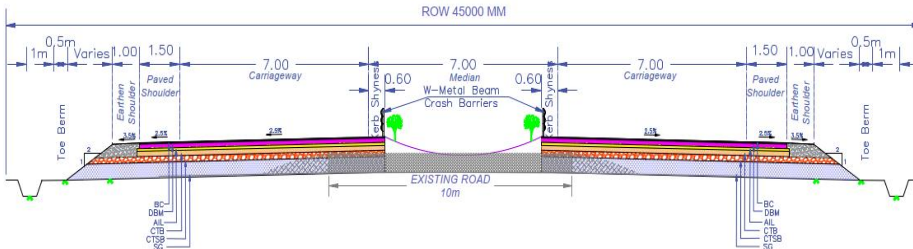
Typical Cross Section for Reconstruction of 4-Lane Divided Highway without Service Roads with Depressed Median (Reconstruction) TCS-02
