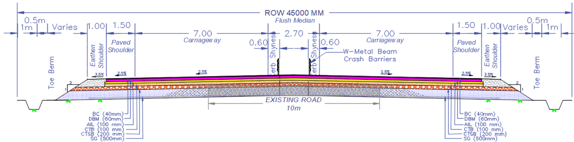
Typical Cross Section for Construction of 4-Lane Divided Highway without Service Roads with Flush Median (Reconstruction) TCS-03
