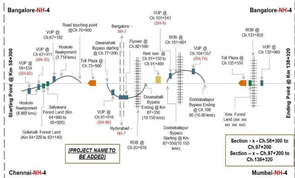
Figure 2: Key plan of existing project road
