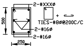
SEC 1-1 (TYP. SEC. OF COL.)
