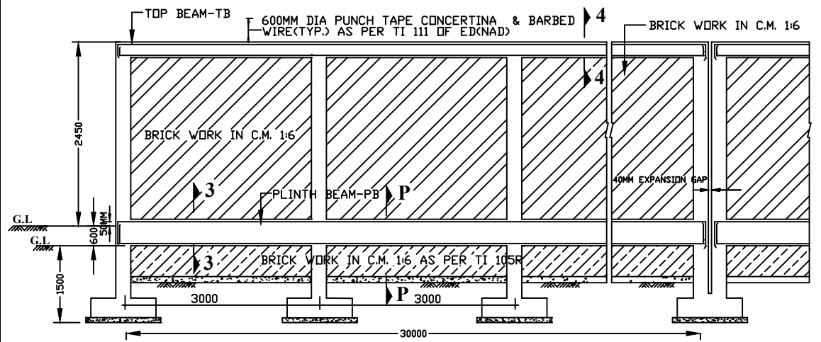
SECTION X - X (COL. REINF. NOT SHOWN)
