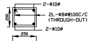
SEC 4-4 (TYP. SEC. OF TB)
