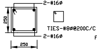
SEC 2-2 (TYP. SEC. OF COL.)
