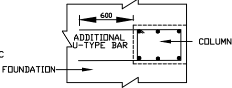
SECTION D-D (PLAN)
