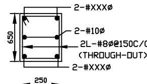
SEC 3-3 (TYP. SEC. OF PB)
