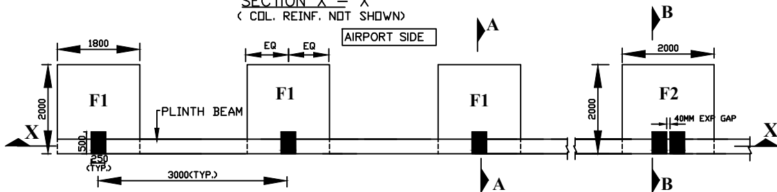
PLAN AT FOUNDATION LEVEL
