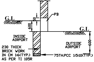
SEC P-P (AS PER T.I 105R)
