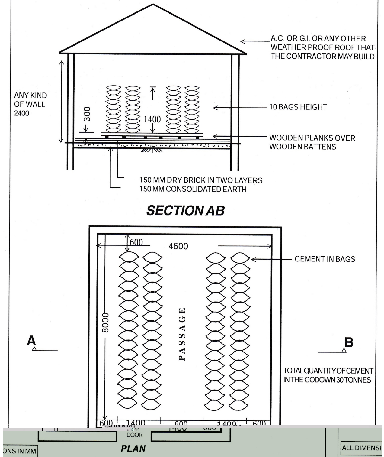
SKETCH OF CEMENT GODOWN
