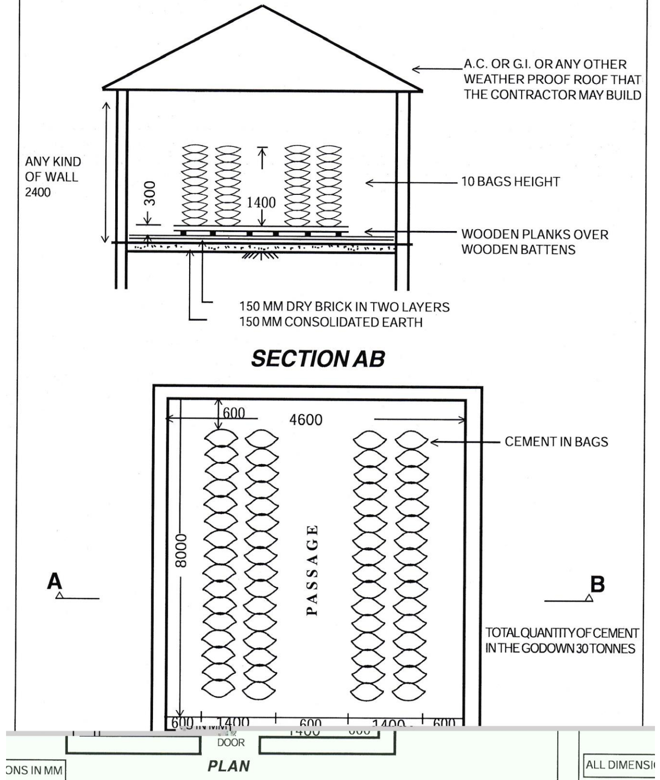
SKETCH OF CEMENT GODOWN
