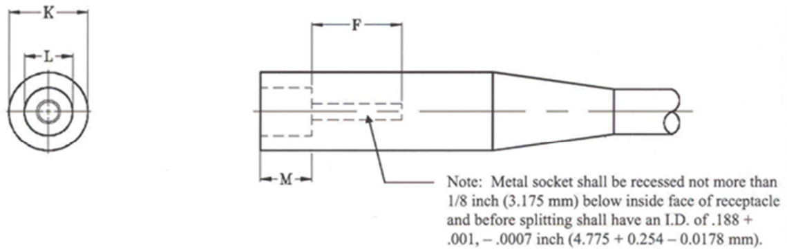
(b) RECEPTACLE – Class A, Type I, Style 9
