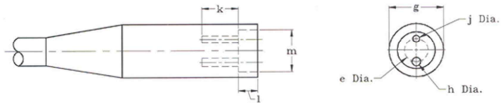
(b) RECEPTACLE - Class A, Type II, Style 7
