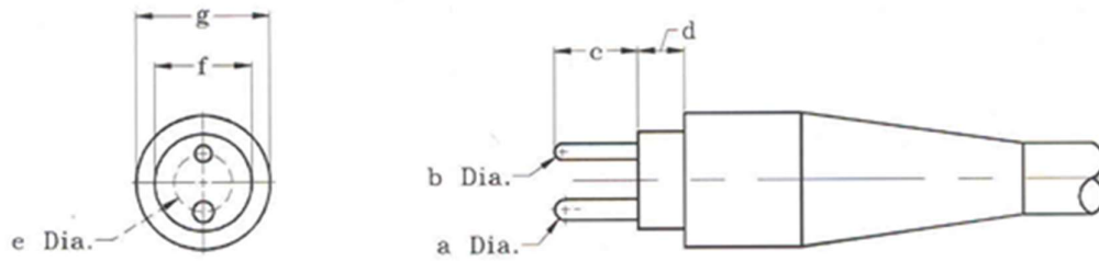
(a) PLUG - Class A, Type II, Style 1
