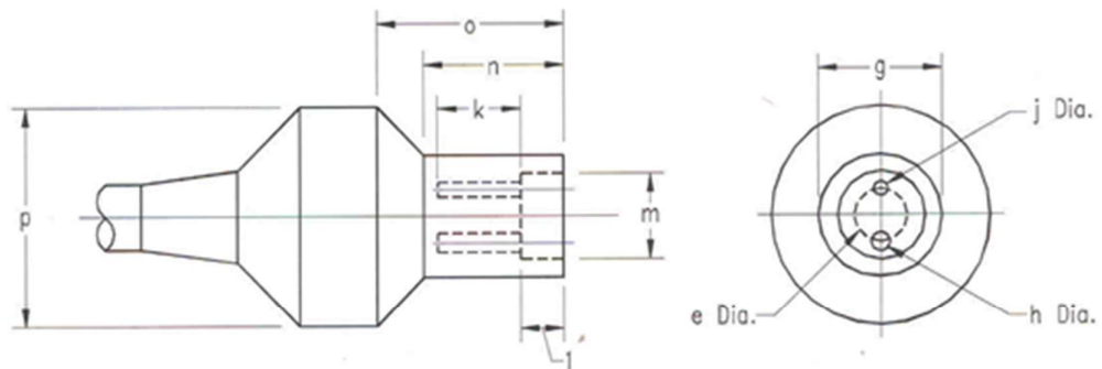
(b) RECEPTACLE - Class A, Type II, Style 7
