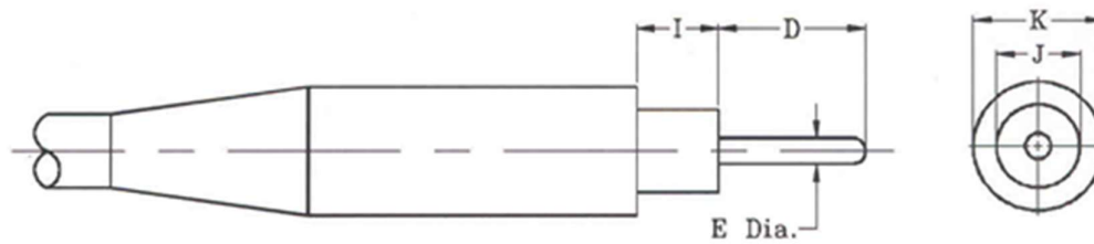
(a) Plug – Class A, Type I, Style 2
