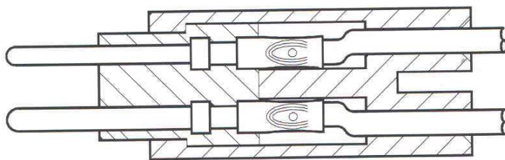
(c) PLUG, a &amp; b Assembled, Style 4
