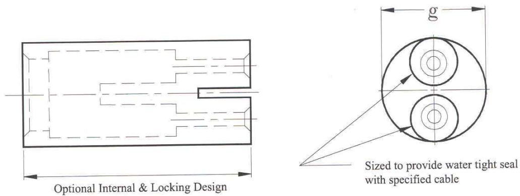
(a) INSERT ASSEMBLY
