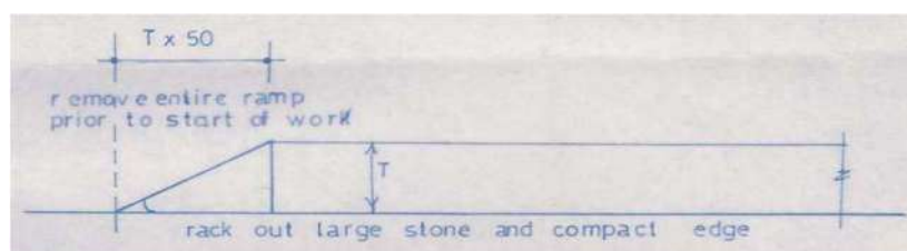
Transverse Temporary Ramp
