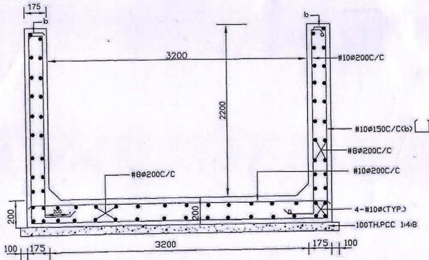
TYPICAL DETAILS OF OPEN DRAIN- PS4 & PN6 (3200Wx2200H) (DETAILS OF OPEN DRAIN- PS3, PN3, PS2, PN2, PN5, CDE1, CDE2 & CDE3 SIMILAR)
